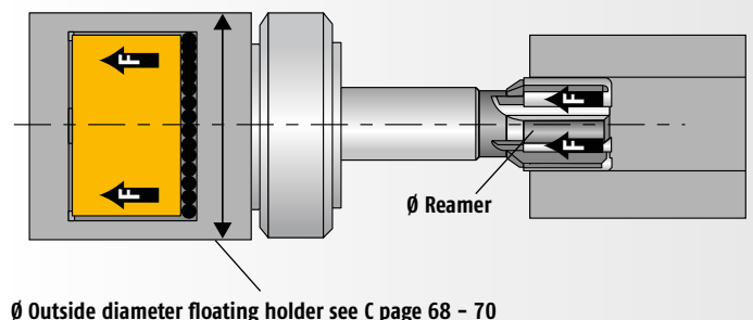
Ø Outside diameter floating holder see C page 68 - 70
